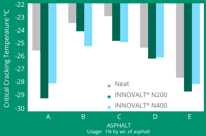
INNOVALT® PPA Impact on Low Temperature Properties
