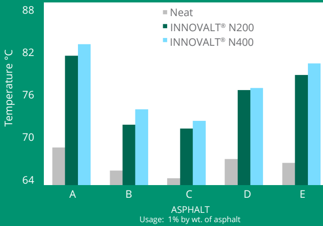
INNOVALT® PPA Impact on High Temperature Properties
